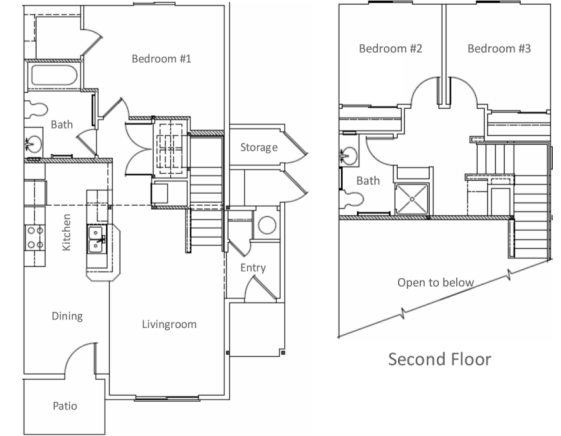
THREE BEDROOM/2BATH 1200 SQFT
